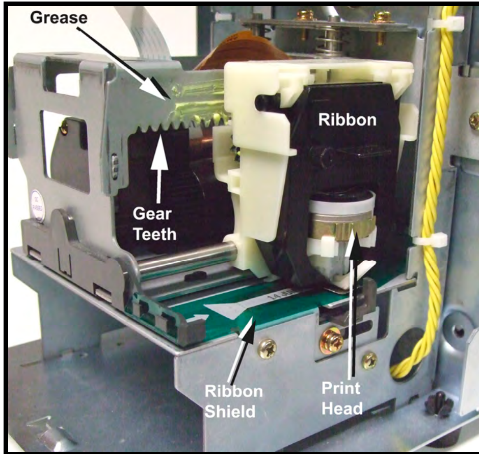
Figure 7-10: Ribbon Carriage Grease
