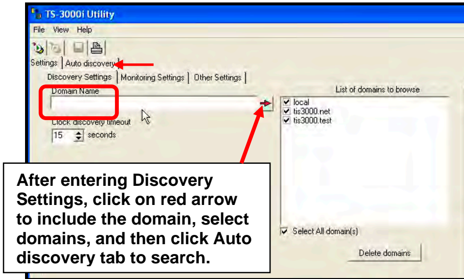
Figure 5-5: Utility Settings
