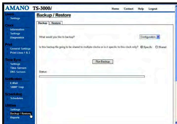
Figure 4-23: Backup Utility
