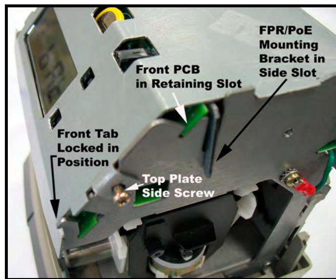
Figure 2-9: Top Plate Installed
