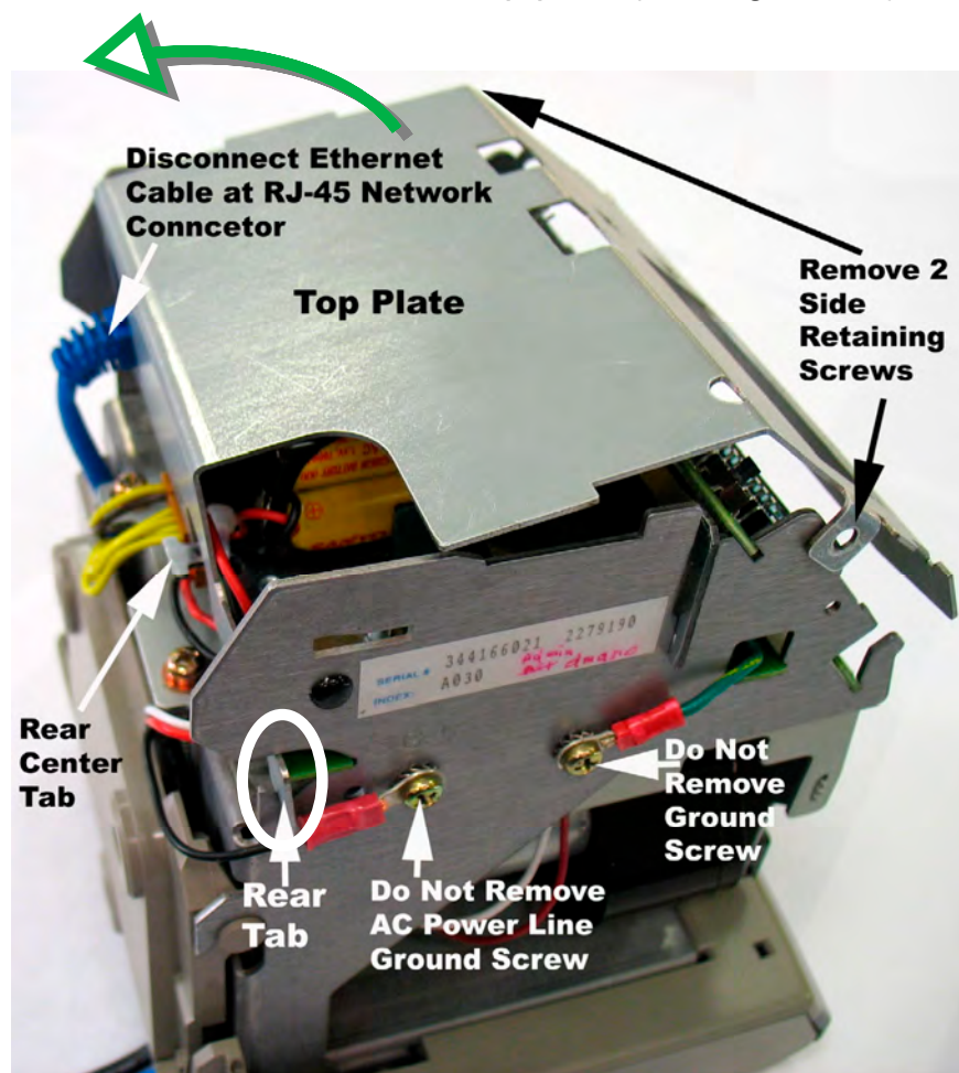
Figure 2-4: Top Plate Removal
