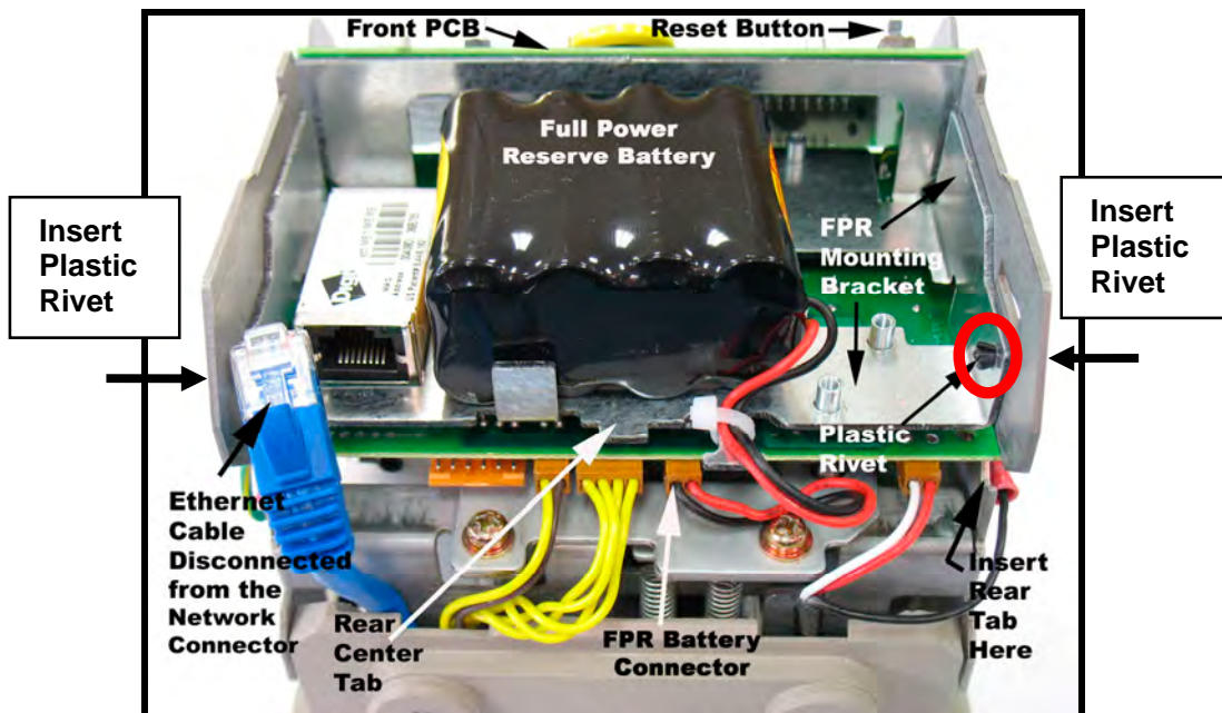
Figure 2-7: TS-3000i Clock Rear View
