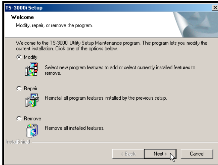
Figure 5-2: Setup Maintenance
