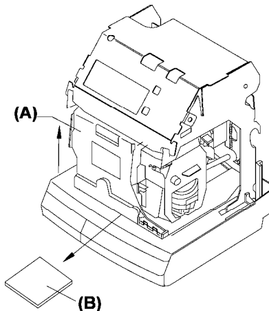
Figure 2-3: TS-3000i Web Clock Packaging
