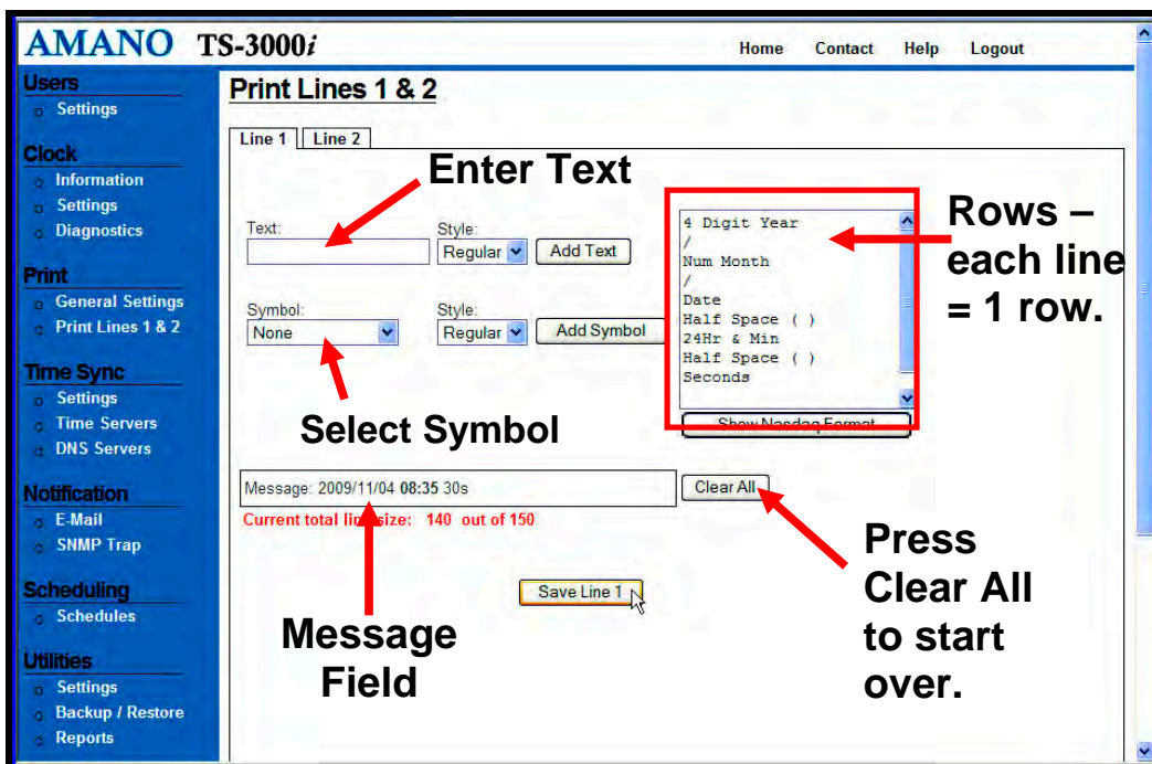
Figure 4-10: Print Lines 1 & 2
