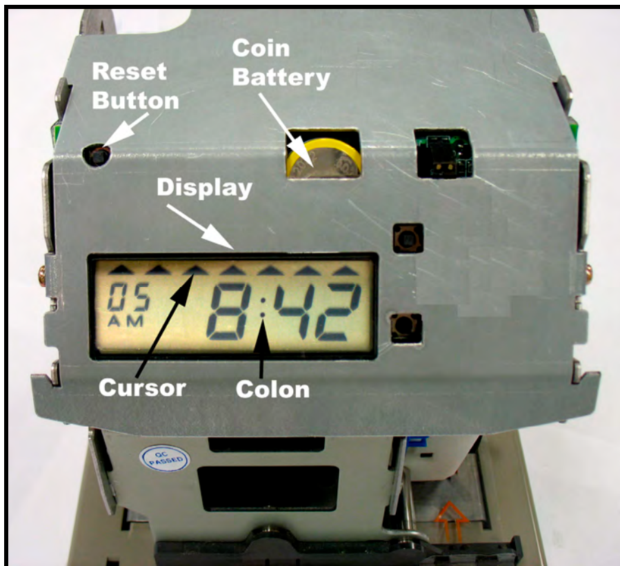
Figure 2-18: TS-3000i Web Clock Front Panel
