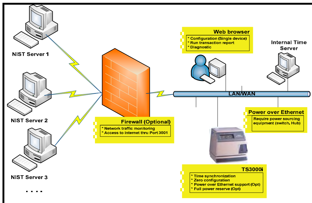
Figure 1-1: TS-3000i Web Clock Time Synchronization
