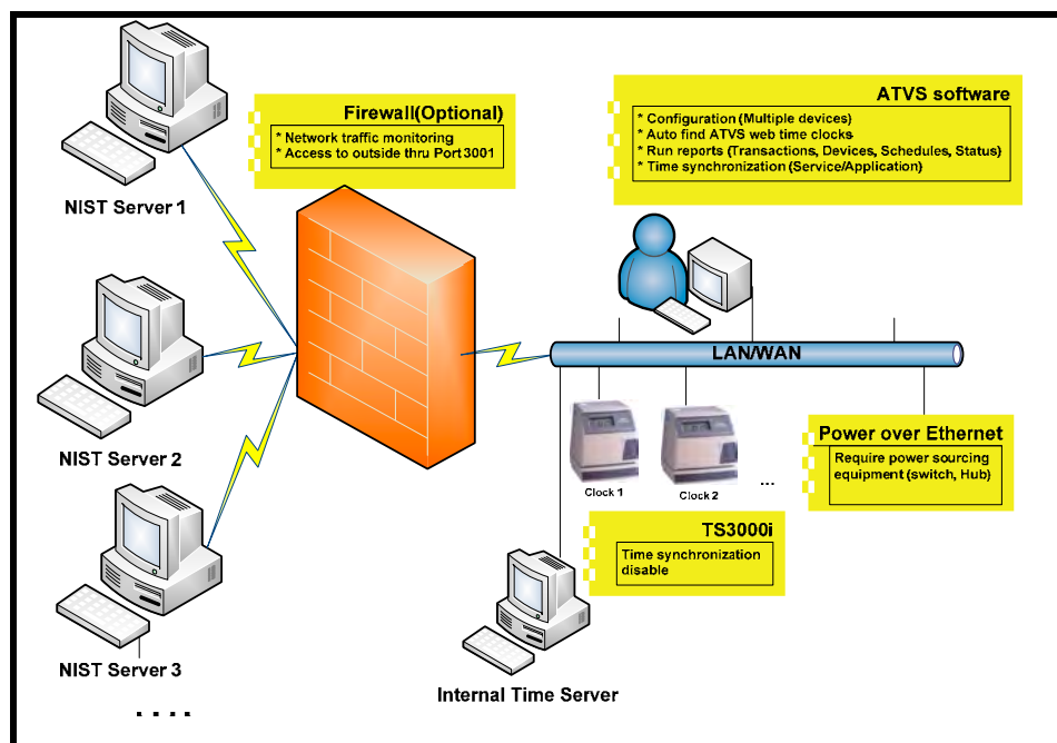
Figure 6-1: ATVS Software & TS-3000i
