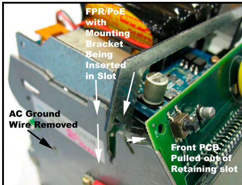
Figure 2-11: Front PCB & Mounting Bracket
