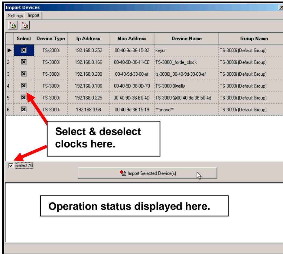
Figure 6-5: Discovered TS-3000i Clocks
