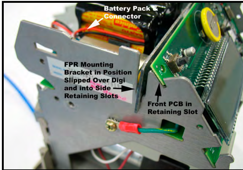
Figure 2-6: Front PCB & FPR Mounting Bracket in Position
