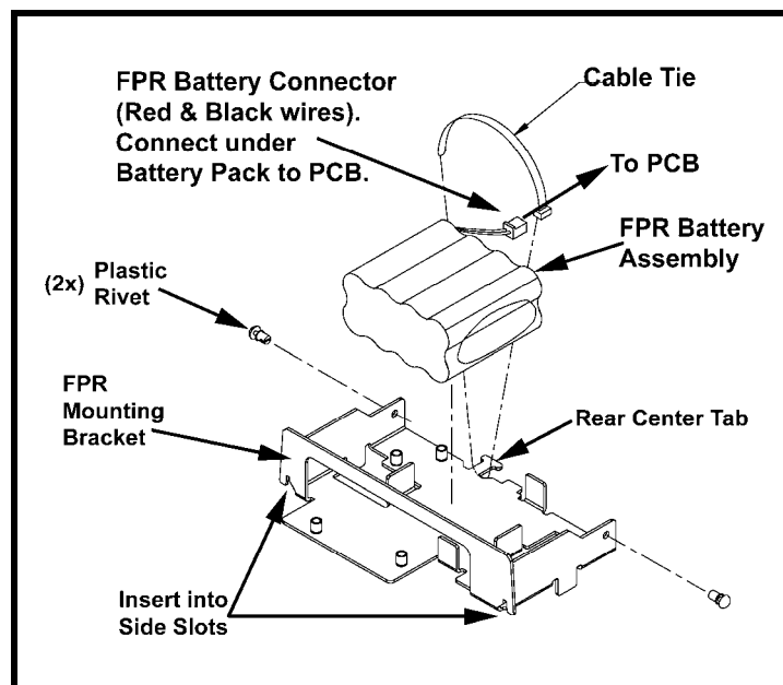
Figure 2-5: FPR & Mounting Bracket
