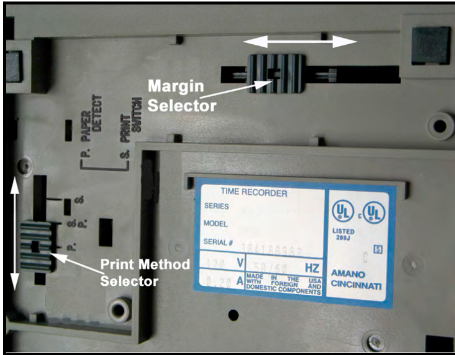
Figure 2-17: TS-3000i Printer Adjustment
