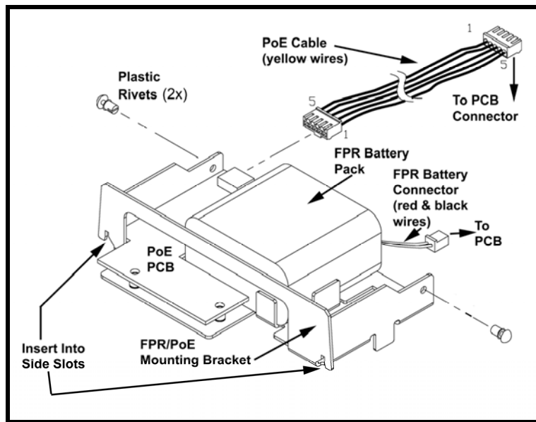
Figure 2-10: PoE/FPR & Mounting Bracket
