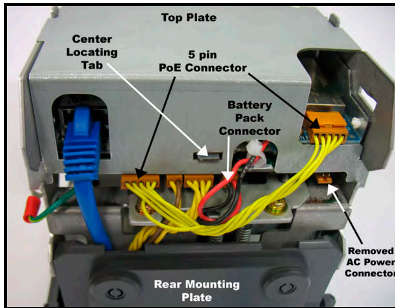
Figure 2-14: PoE & FPR Connectors
